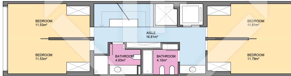
Fourth floor
