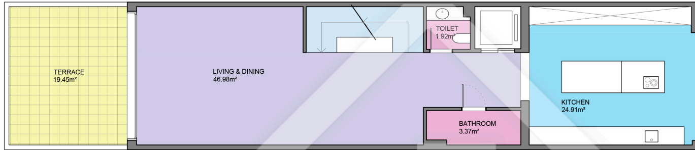
Second floor
